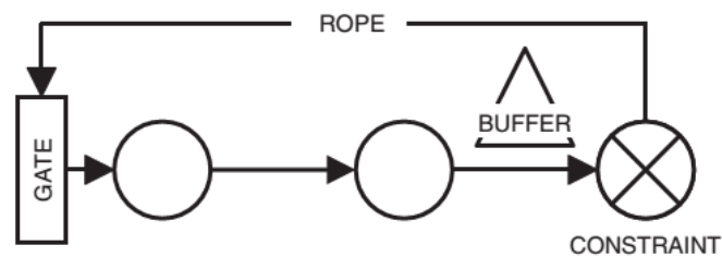
Fig. 2. The Drum- buffer- rope method (Watson and Patti, 2008)
